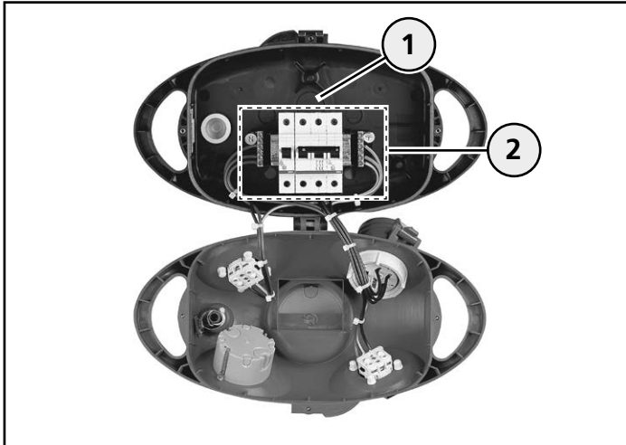
Connecting the supply line (example AirKRAFT®)
